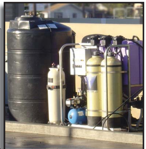
Hydro Loop® Stationary Wastewater Treatment
